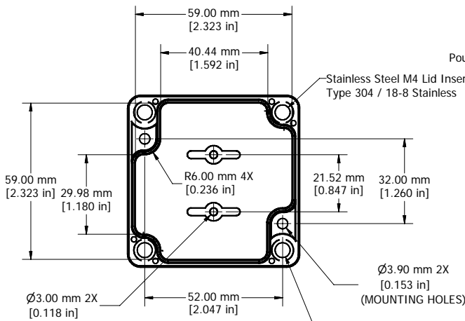
BOX - INSIDE
